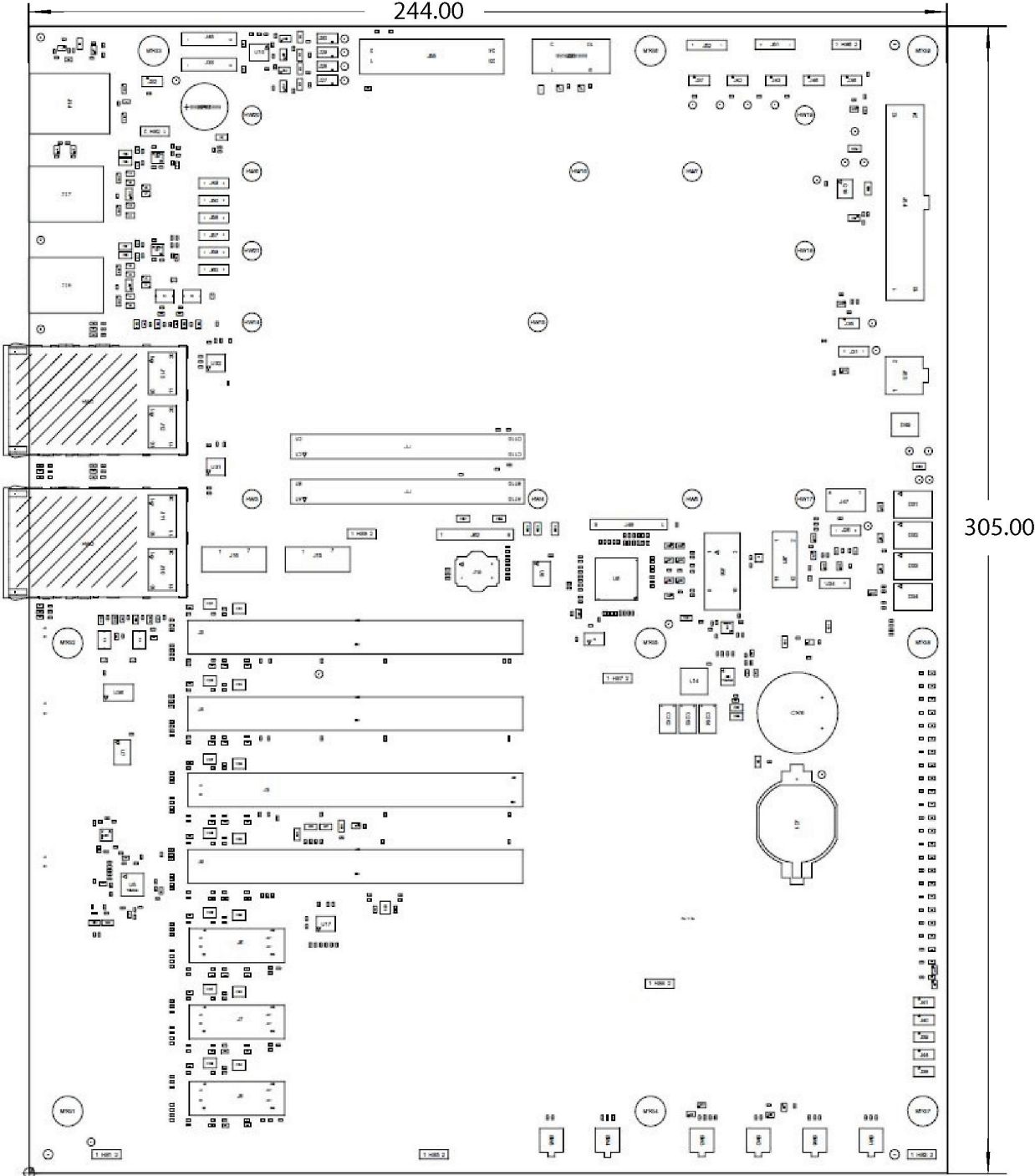
Figure 5: Board Dimensions
