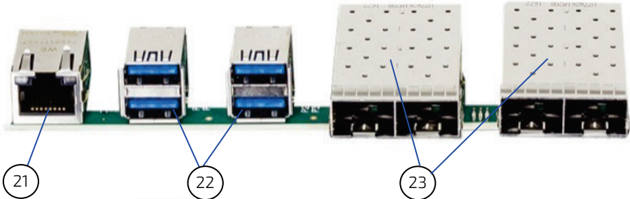
Figure 4: Front Panel
