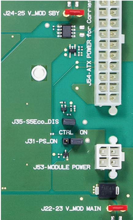
Figure 24: Jumper J22-23, J24-25, J31, J35
