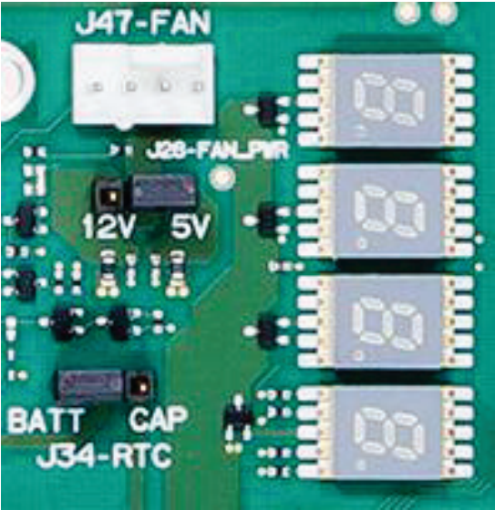
Figure 25: Jumper J26, J34
