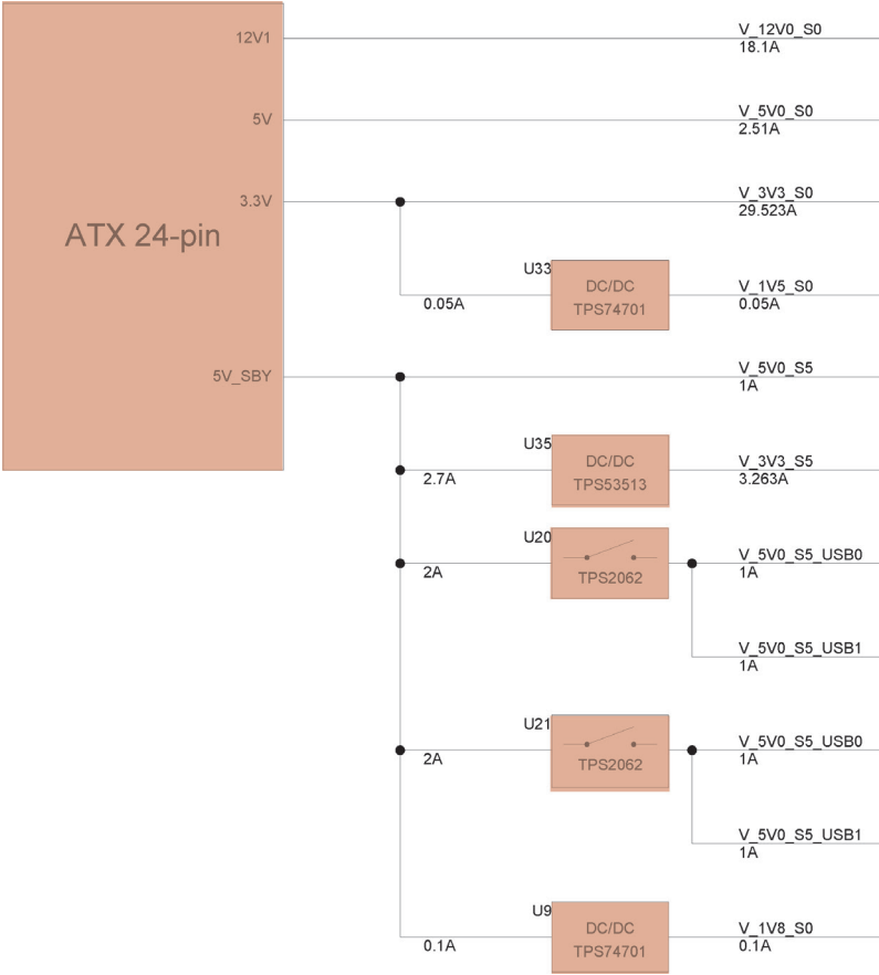
Figure 19: Power Supply ATX 24-pin for Carrier Board (J54)
