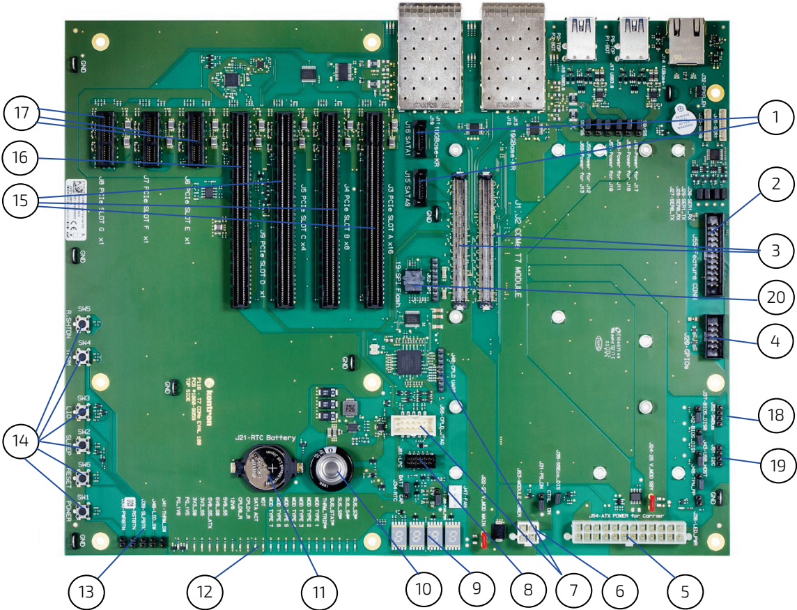
Figure 3: Top View of COMe Eval Carrier T7
