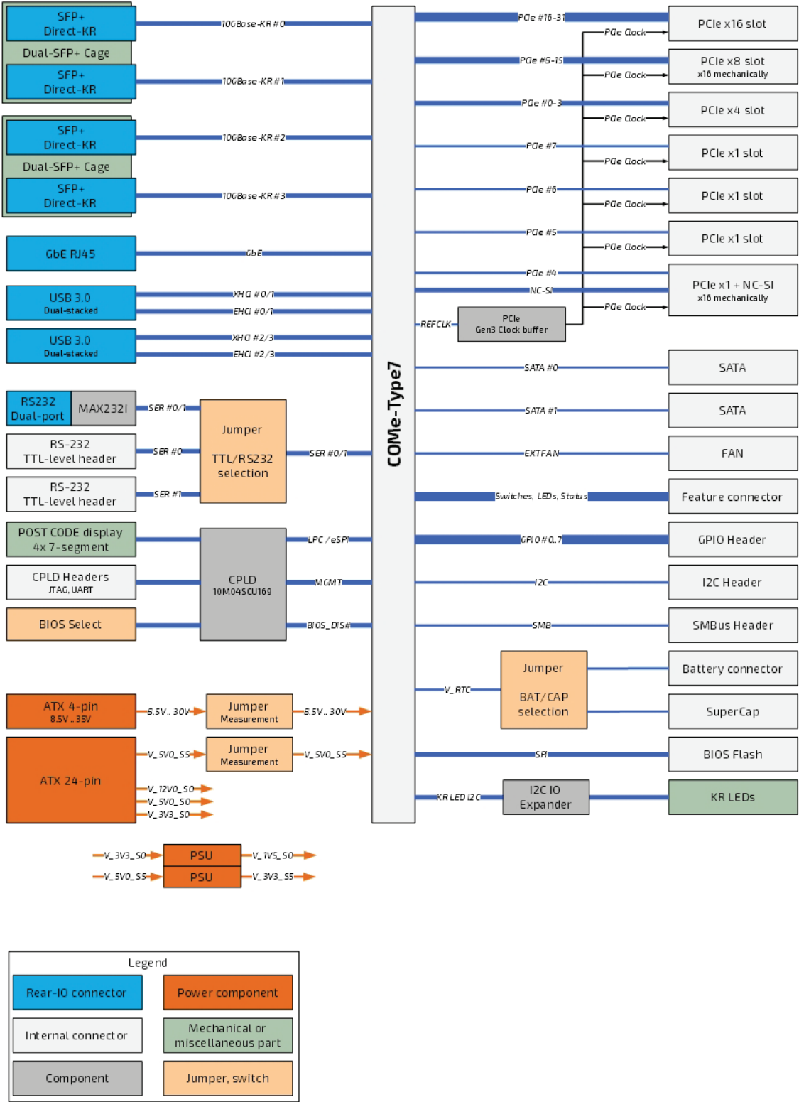
Figure 2: Block Diagram COME-Type7 Validation/Evaluation carrier
