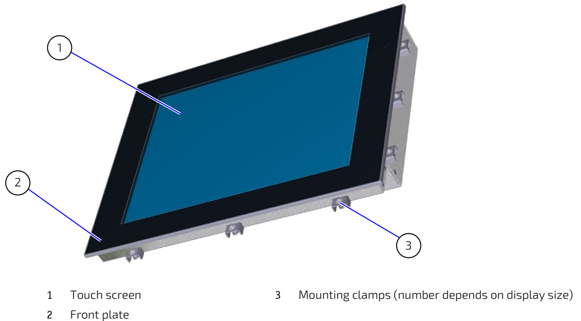
Figure 5: Front Side – FlatView (built-in)/FlatView STS
