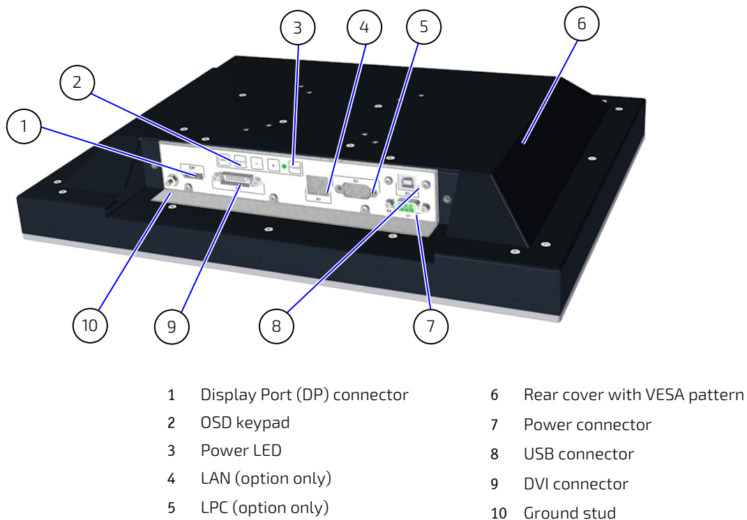
Figure 4: Rear Panel – FlatView (VESA)
