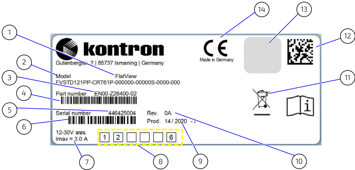
Figure 2: Type Label
