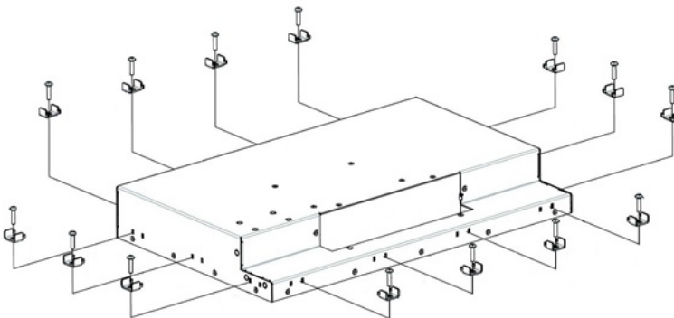
Figure 13: Clamping Bracket Positions
