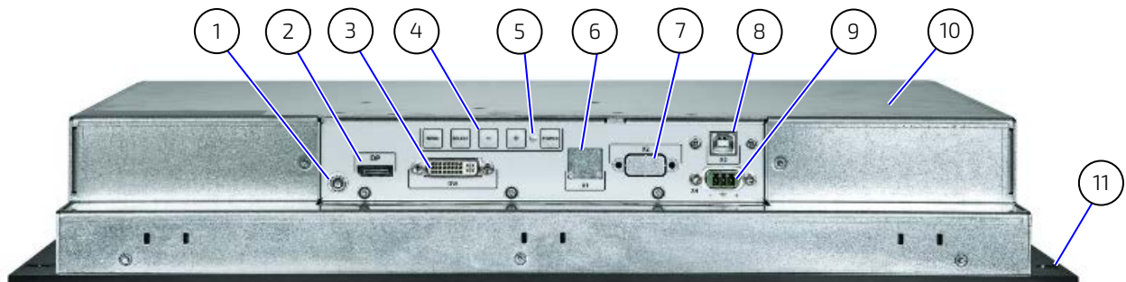
Figure 8: Rear Panel – FlatView RCK
